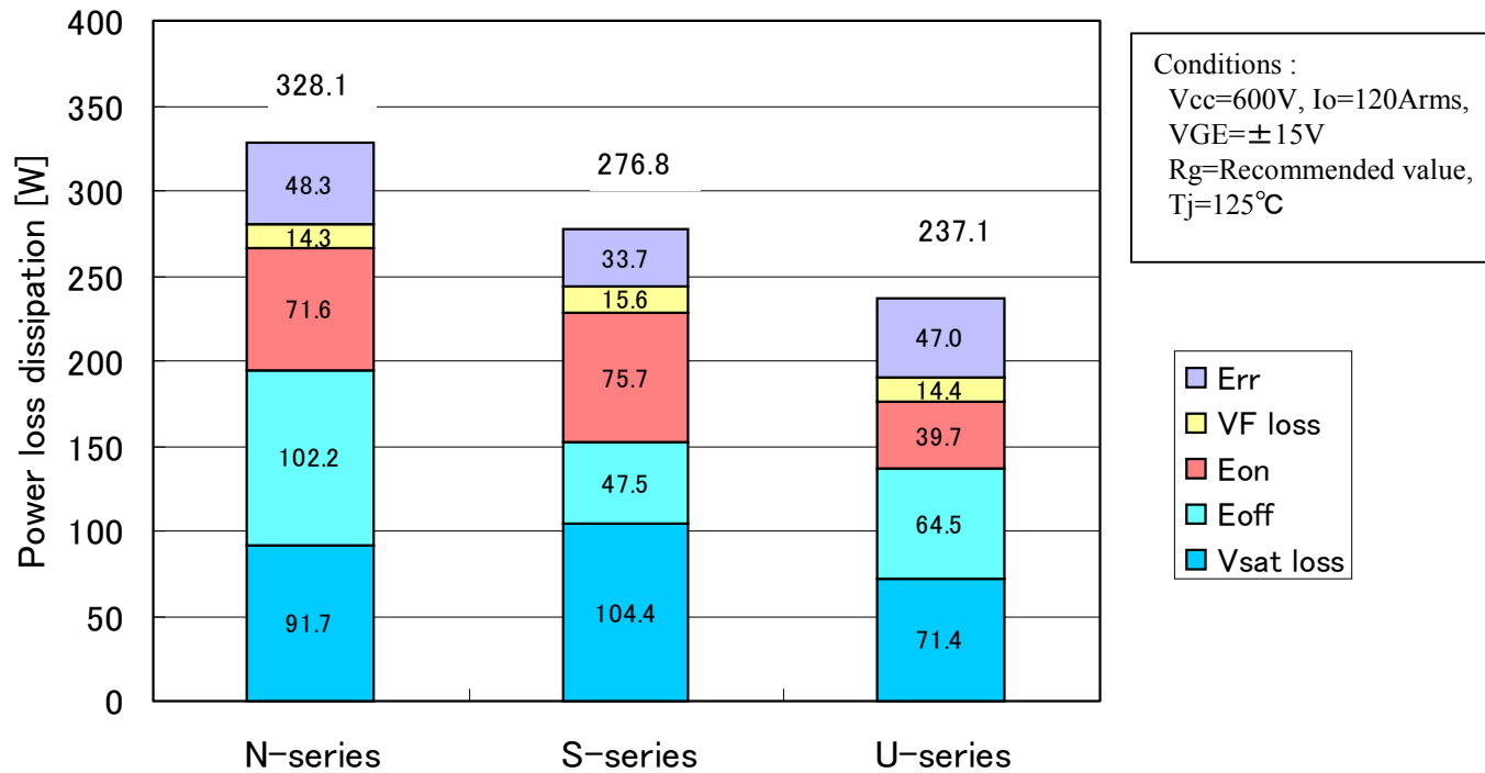
1200V/200A Comparison of power dissipation loss
